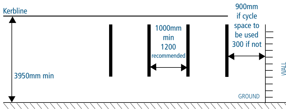
ARRANGEMENT PARALLEL TO WALL
