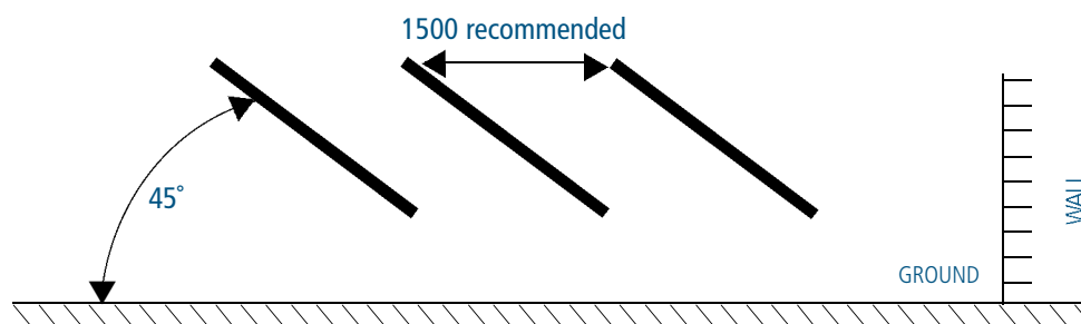
ARRANGEMENT AT 45° TO WALL
